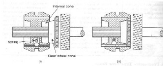
Synchromesh unit
