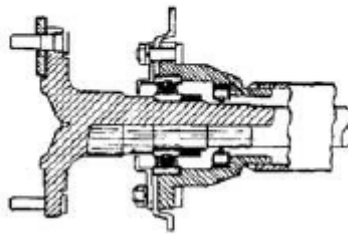
Fig..Semi-floatingball-race-bearing.
